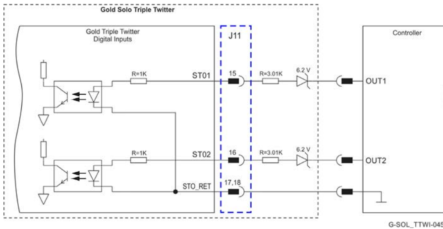
Figure 39: STO Input Connection – PLC (24V Logic)
