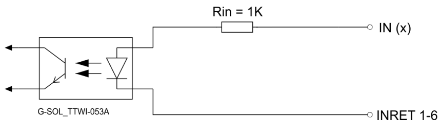
Figure 30: Digital Input 5V Logic Schematic
