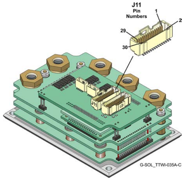
J11 I/O and Communication Connector
